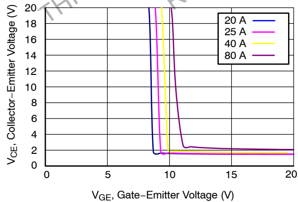
Figure 5. Saturation Voltage vs. V_{GE} ( 25^\circ\text{C} )
