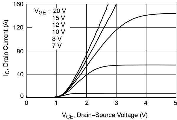
Figure 1. Typical Output Characteristics ( 25^\circ\text{C} )
