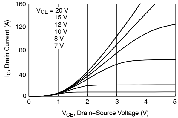
Figure 2. Typical Output Characteristics ( 175^\circ\text{C} )
