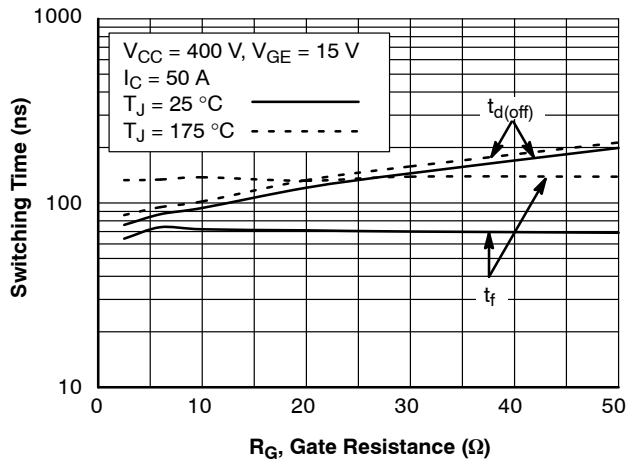
Figure 9. Turn-off Characteristics vs. Gate Resistance
