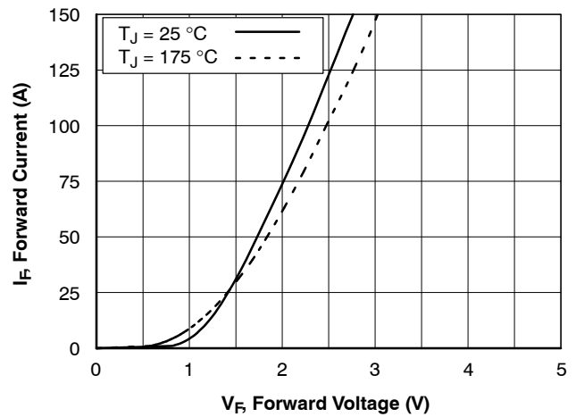
Figure 14. Forward Characteristics
