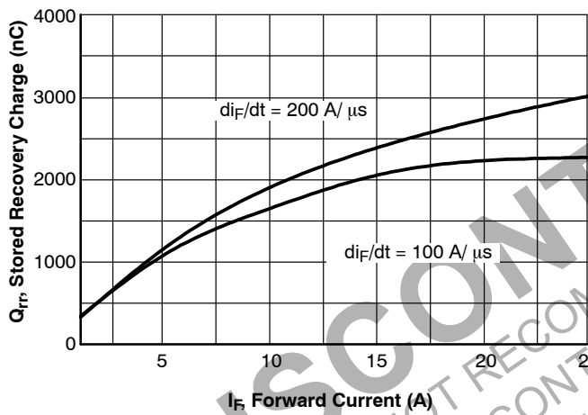
Figure 20. Stored Charge
