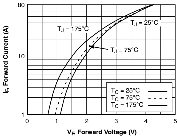
Figure 17. Forward Characteristics
