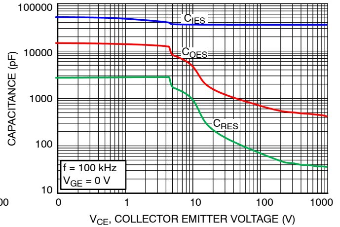
Figure 9. Capacitance Characteristics
